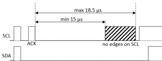
Figure 19 Stop condition after critical time window
